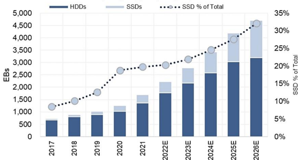
HDD and SSD Capacity Shipped (Exabytes); SSDs % of Total
